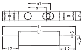
Multiple retaining plates
